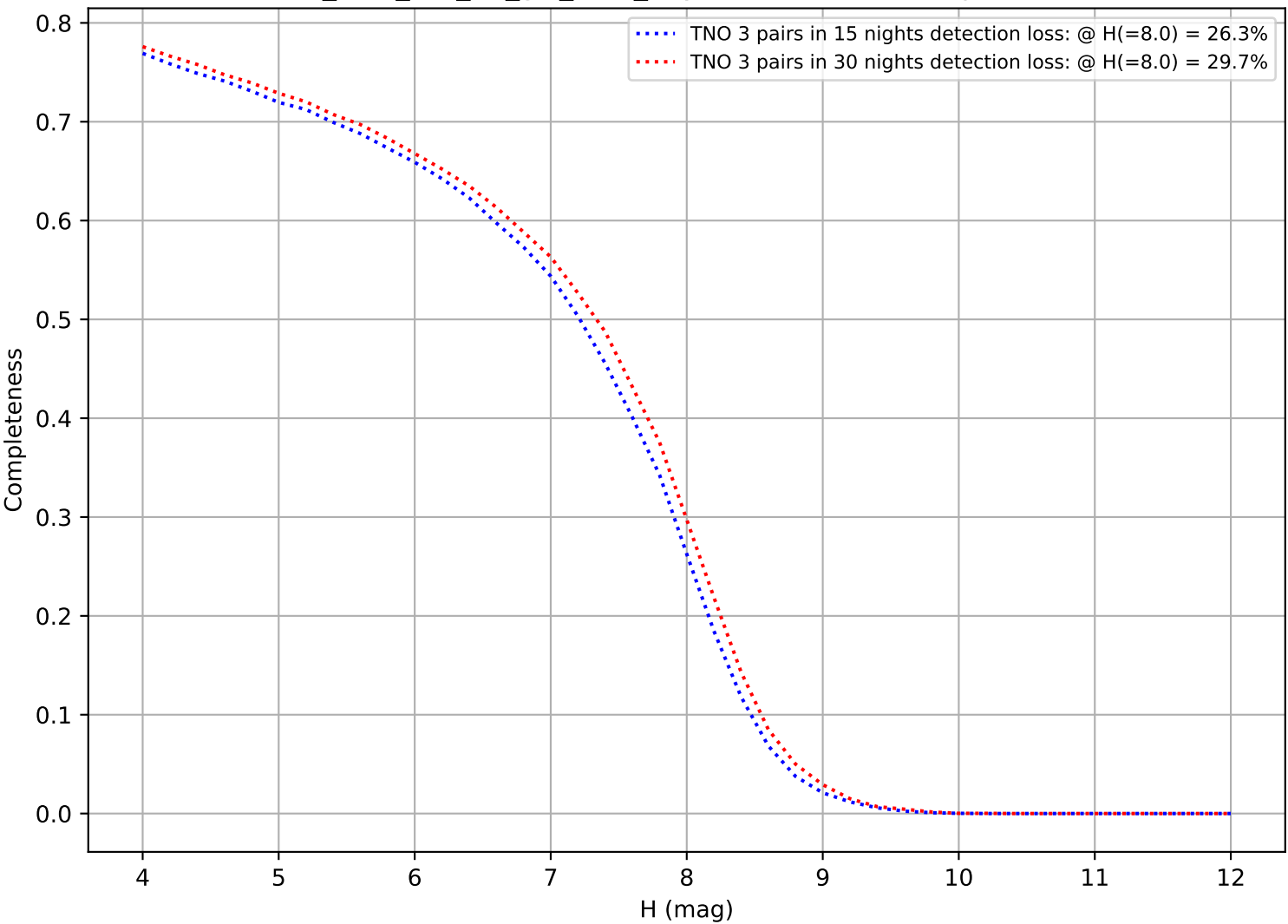
too_elab_r64_d2_giz_v3.4_10yrs: DifferentialCompleteness
