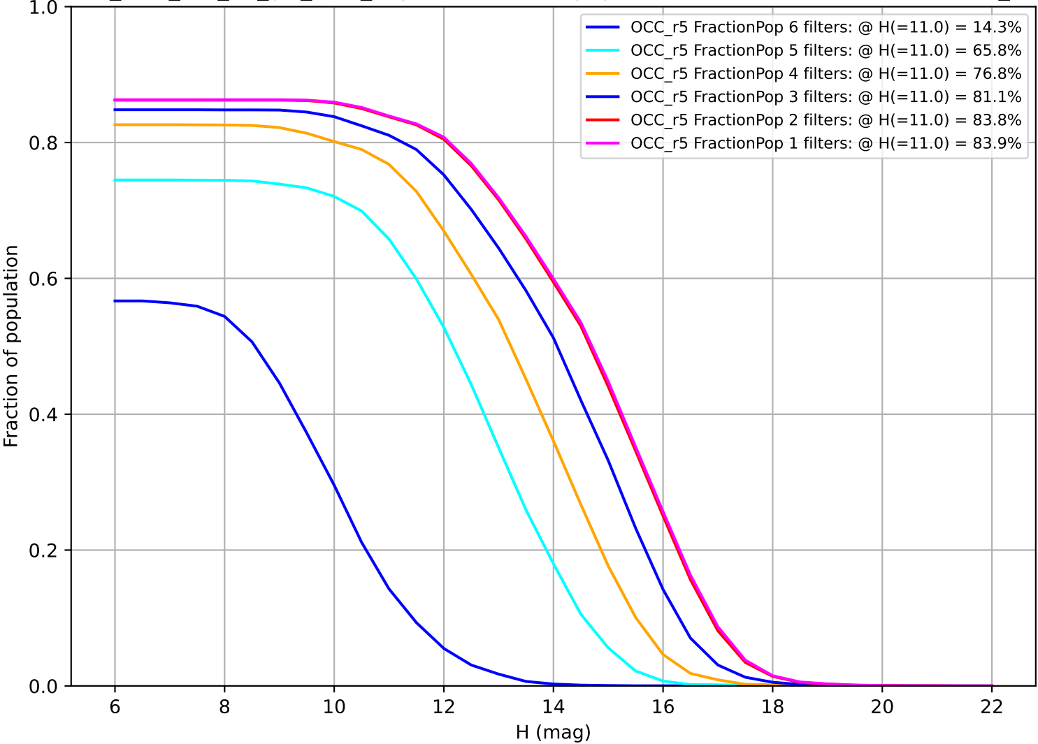
too_elab_r64_d2_giz_v3.4_10yrs: Fraction of population with colors in X filters OCC_r5
