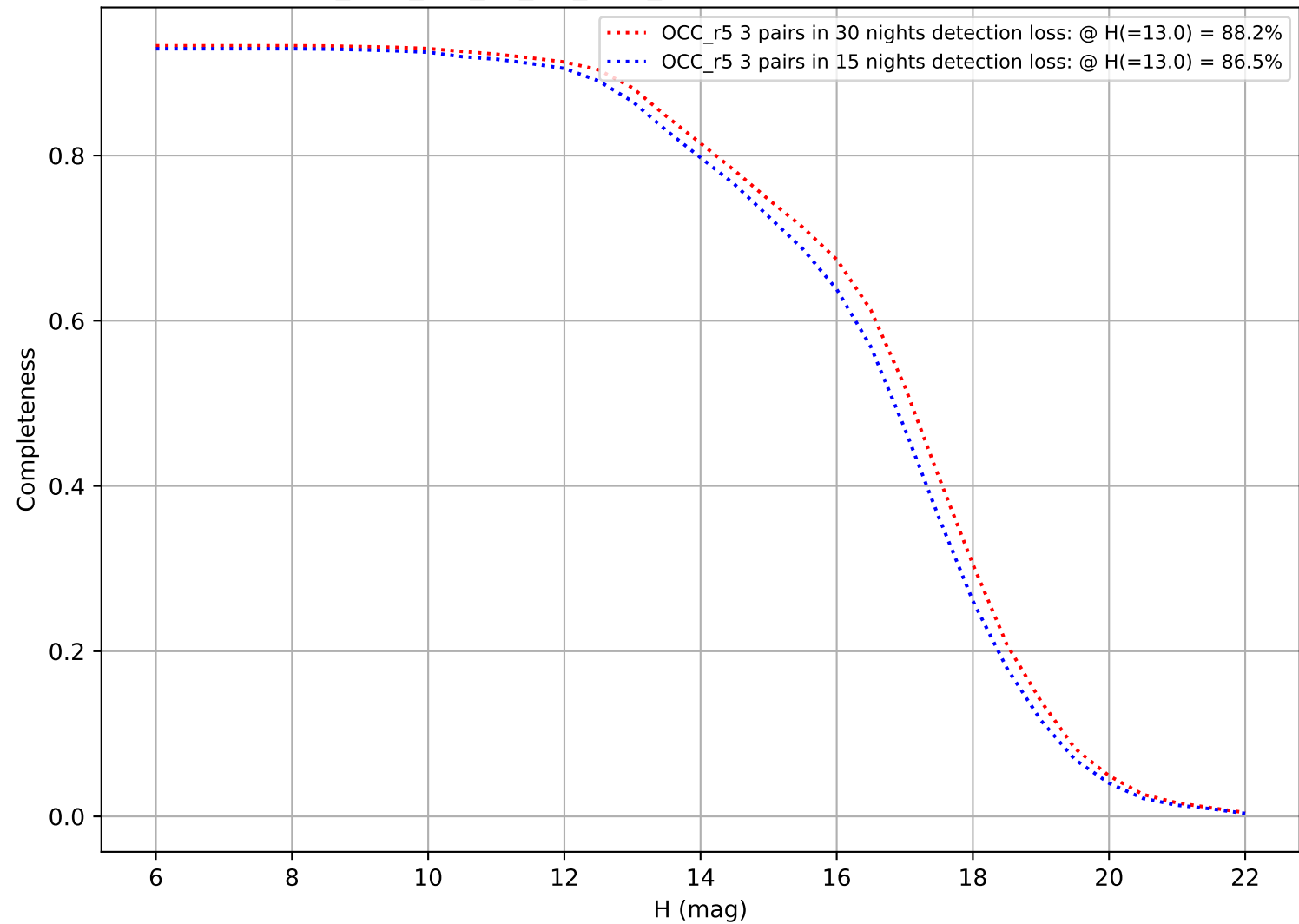
too_elab_r64_d2_giz_v3.4_10yrs: DifferentialCompleteness
