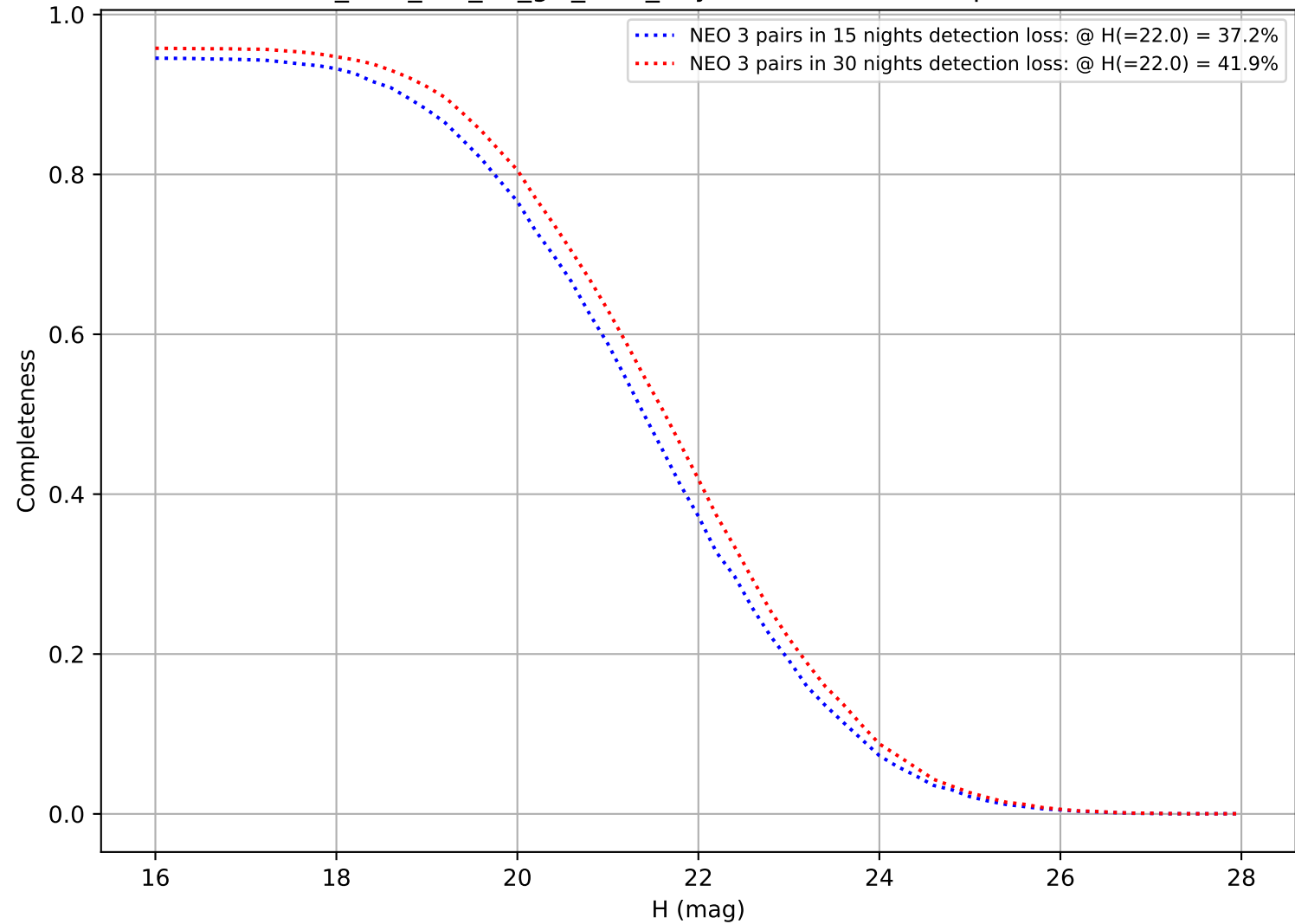
too_elab_r64_d2_giz_v3.4_10yrs: DifferentialCompleteness
