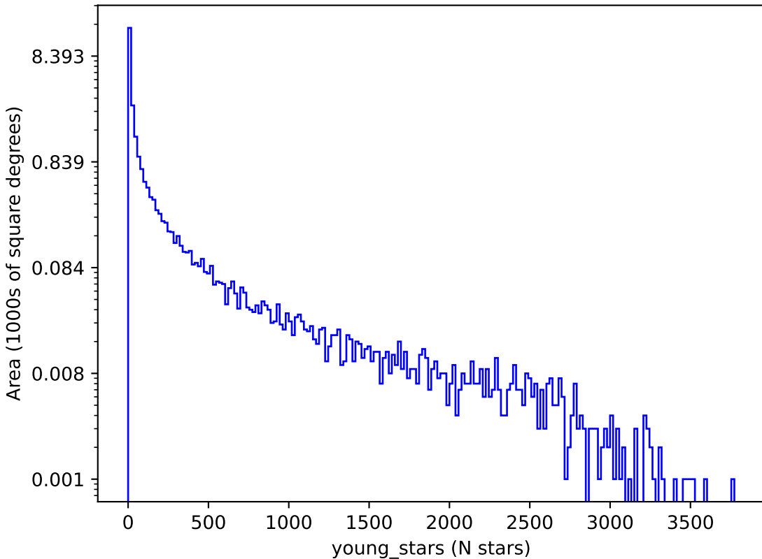
too_elab_r64_d2_giz_v3.4_10yrs : young_stars
