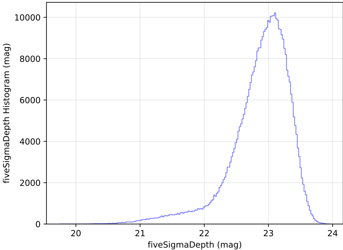
too_elab_r64_d2_giz_v3.4_10yrs z: fiveSigmaDepth Histogram
