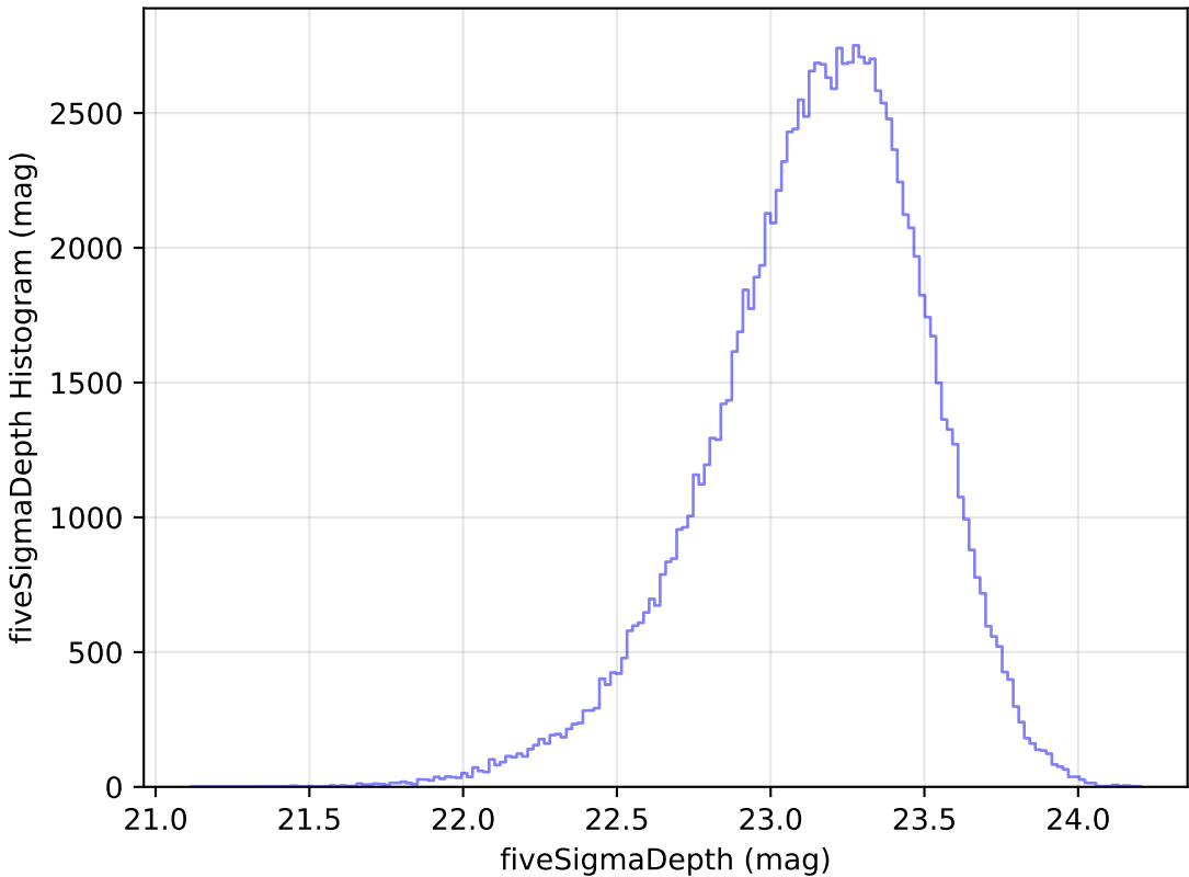
too_elab_r64_d2_giz_v3.4_10yrs u: fiveSigmaDepth Histogram
