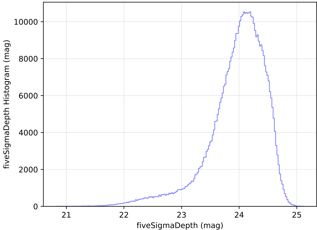
too_elab_r64_d2_giz_v3.4_10yrs r: fiveSigmaDepth Histogram
