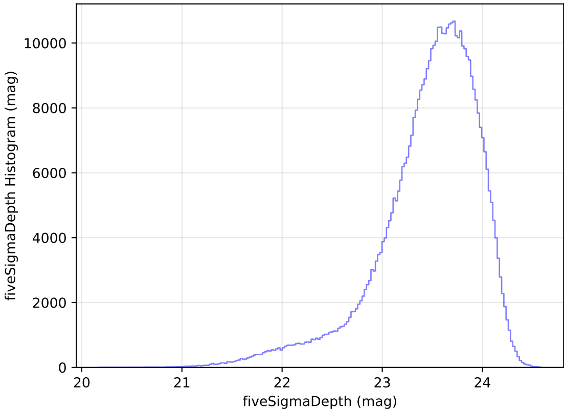
too_elab_r64_d2_giz_v3.4_10yrs i: fiveSigmaDepth Histogram
