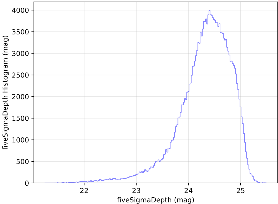
too_elab_r64_d2_giz_v3.4_10yrs g: fiveSigmaDepth Histogram
