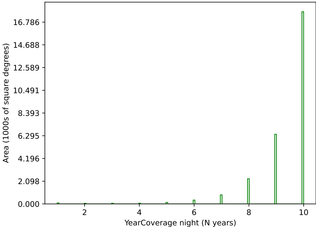
too_elab_r64_d2_giz_v3.4_10yrs g band: YearCoverage night
