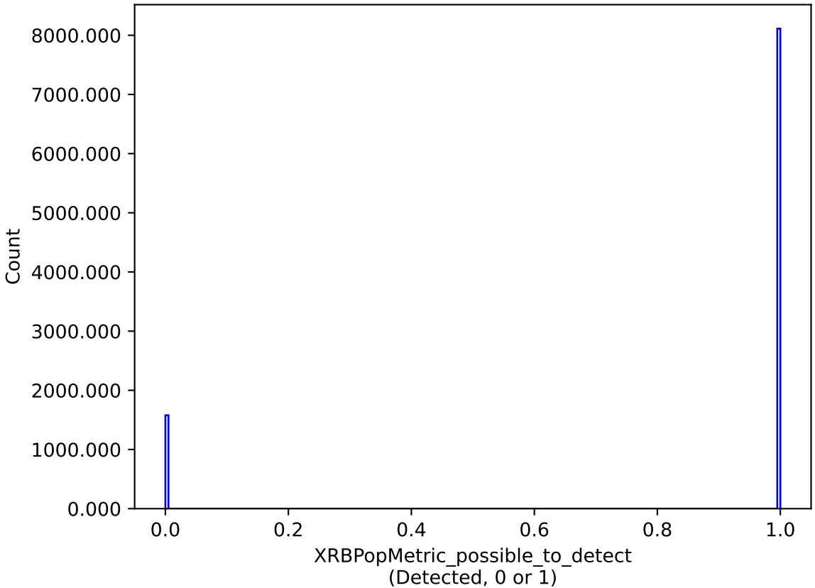
too_elab_r64_d2_giz_v3.4_10yrs : XRBPoMetric_possible_to_detect
