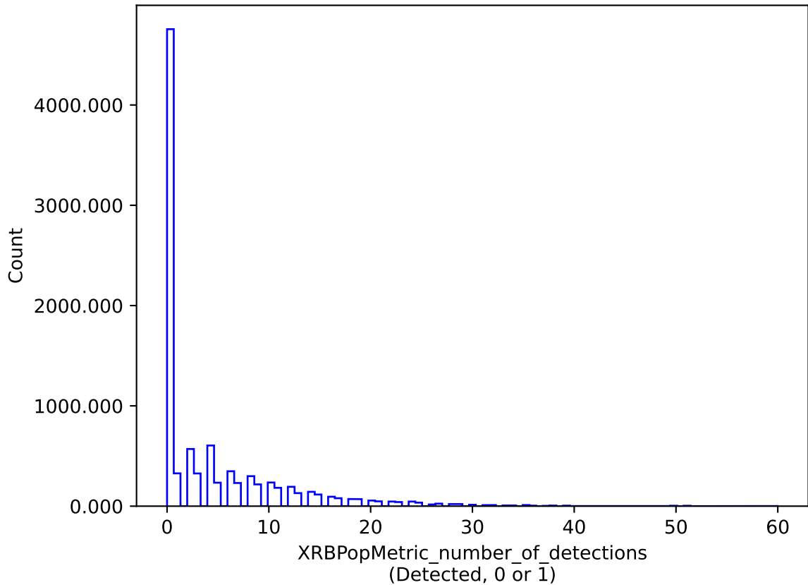
too_elab_r64_d2_giz_v3.4_10yrs : XRBPoMetric_number_of_detections
