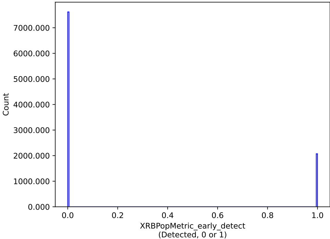
too_elab_r64_d2_giz_v3.4_10yrs : XRBPoMetric_early_detect
