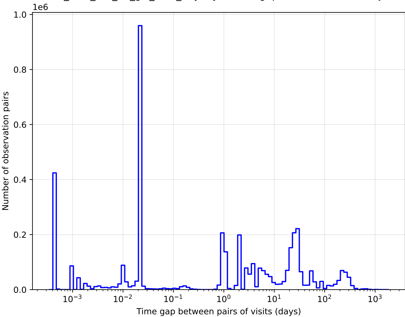
too_elab_r64_d2_giz_v3.4_10yrs y band: Tgaps observationStartMJD
