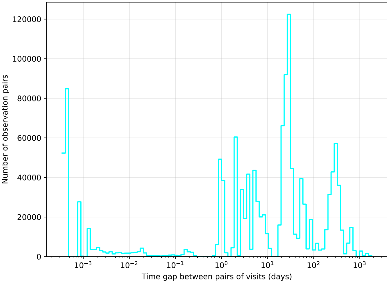
too_elab_r64_d2_giz_v3.4_10yrs u band: Tgaps observationStartMJD
