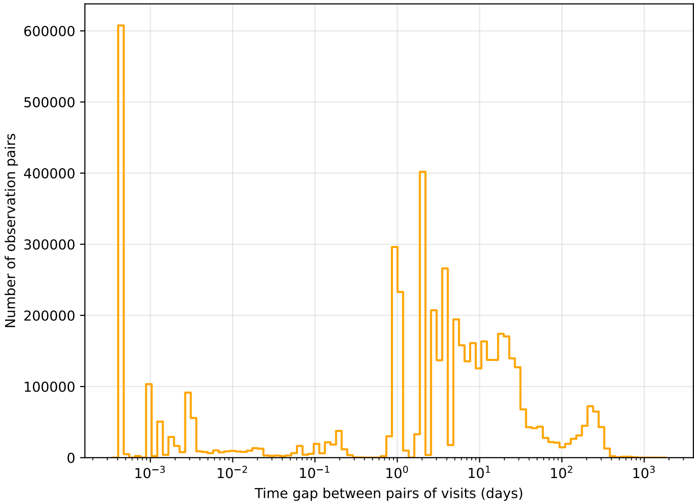
too_elab_r64_d2_giz_v3.4_10yrs r band: Tgaps observationStartMJD
