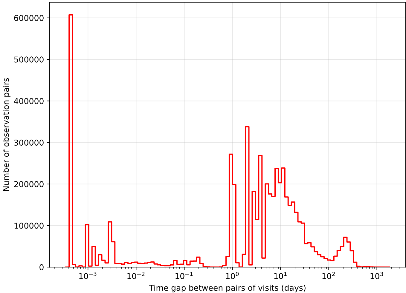
too_elab_r64_d2_giz_v3.4_10yrs i band: Tgaps observationStartMJD
