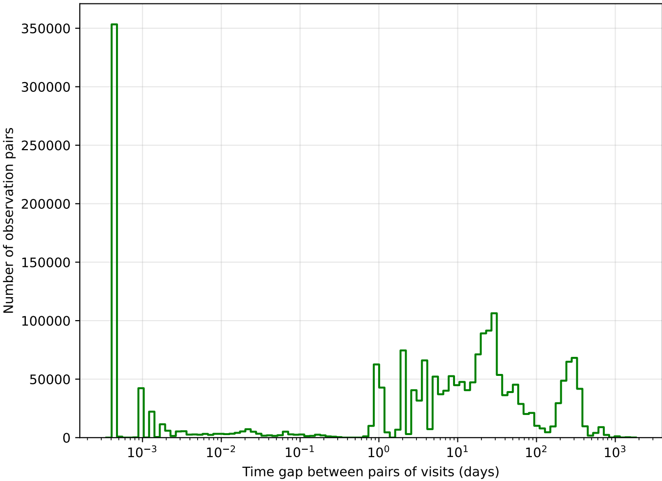
too_elab_r64_d2_giz_v3.4_10yrs g band: Tgaps observationStartMJD
