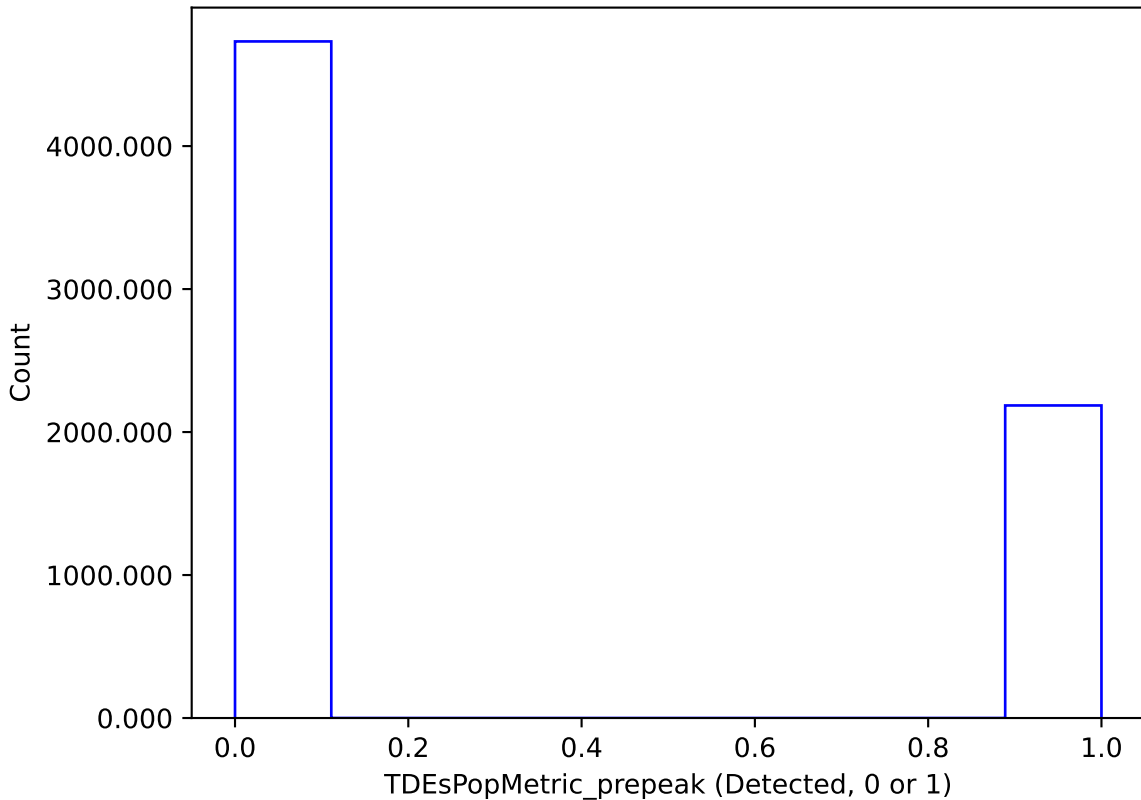
too_elab_r64_d2_giz_v3.4_10yrs : TDEsPopMetric_prepeak
