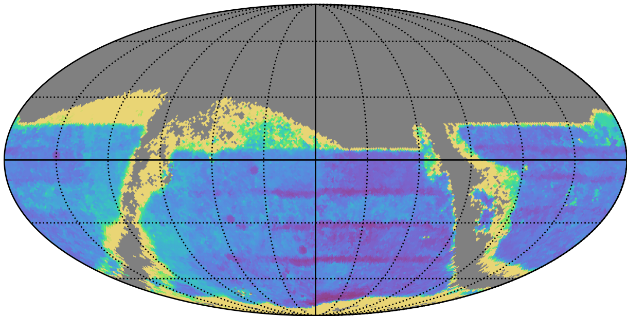
too_elab_r64_d2_giz_v3.4_10yrs : TDC_accuracy
