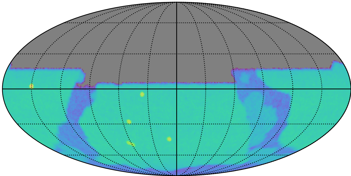
too_elab_r64_d2_giz_v3.4_10yrs u: SurfaceBrightLimit
