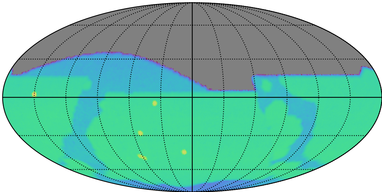
too_elab_r64_d2_giz_v3.4_10yrs r: SurfaceBrightLimit
