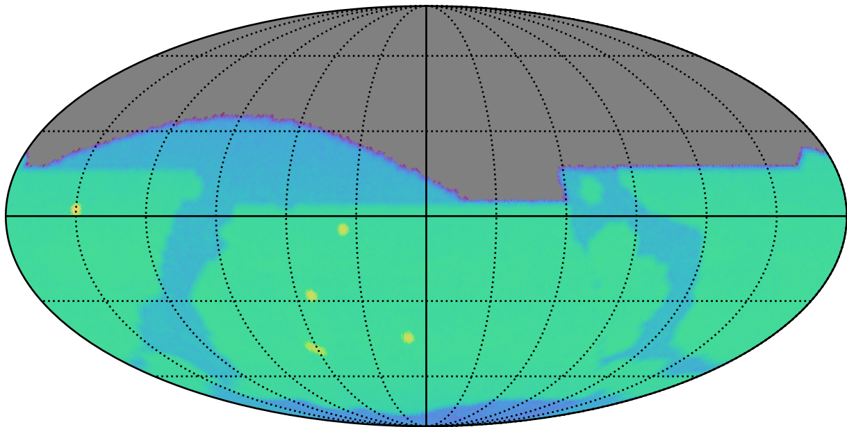
too_elab_r64_d2_giz_v3.4_10yrs i: SurfaceBrightLimit
