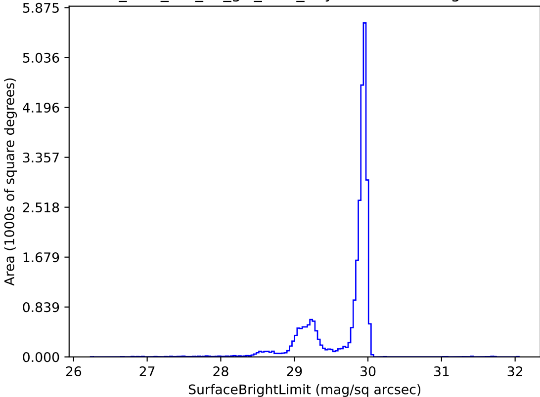
too_elab_r64_d2_giz_v3.4_10yrs i: SurfaceBrightLimit
