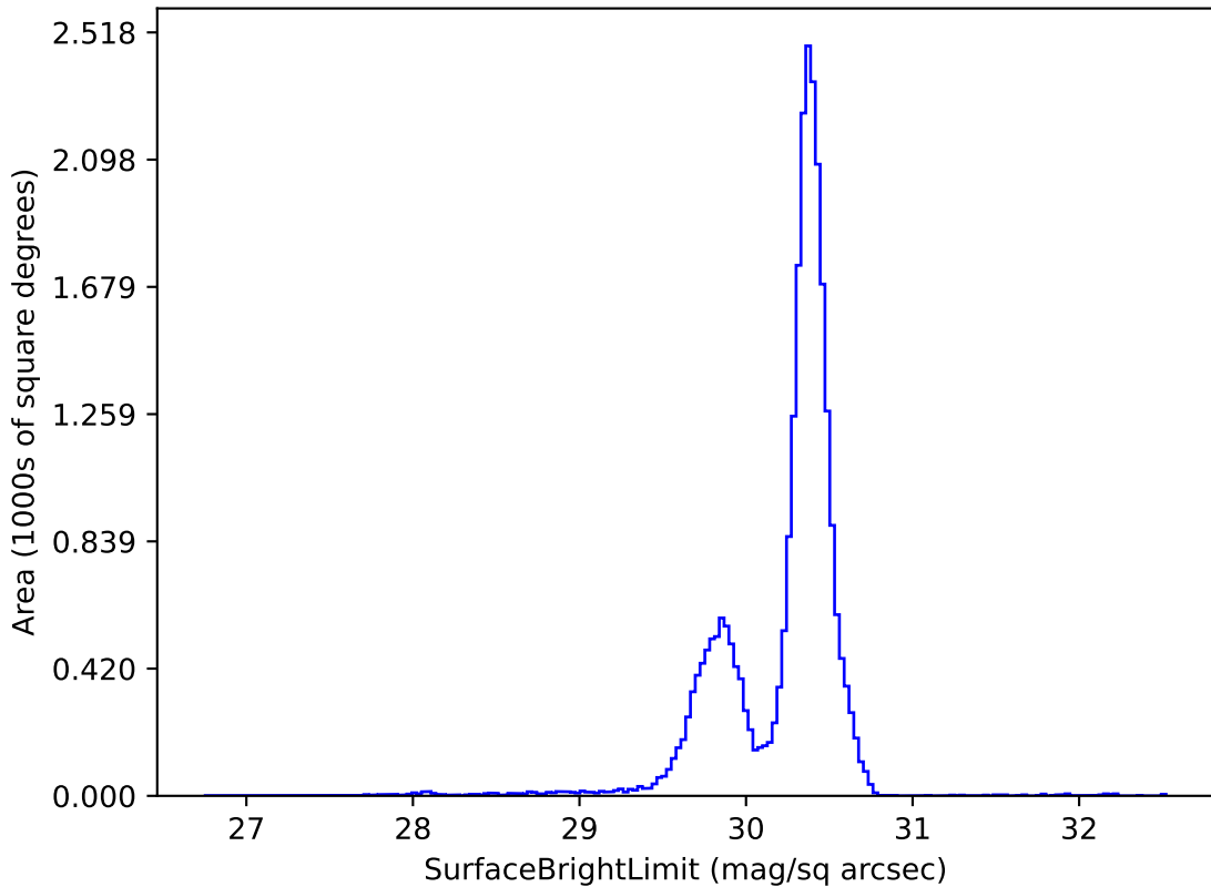
too_elab_r64_d2_giz_v3.4_10yrs g: SurfaceBrightLimit
