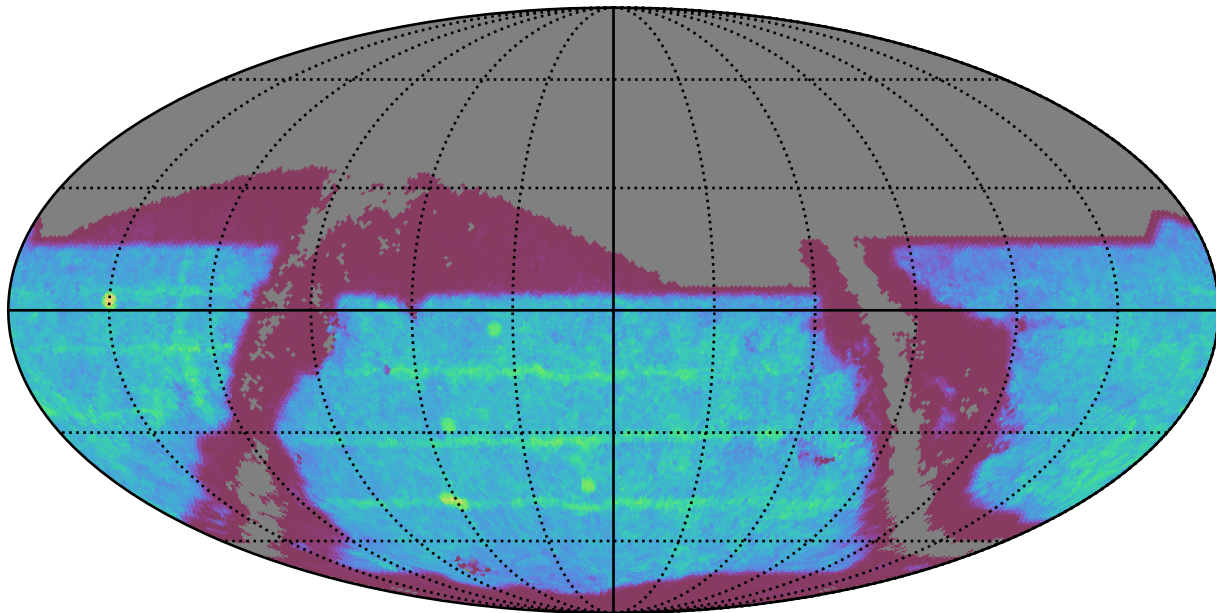
too_elab_r64_d2_giz_v3.4_10yrs : SNSLMetric
