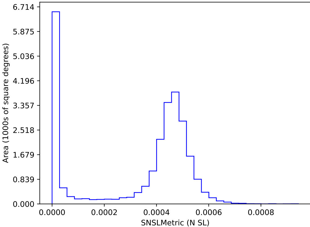
too_elab_r64_d2_giz_v3.4_10yrs : SNSLMetric
