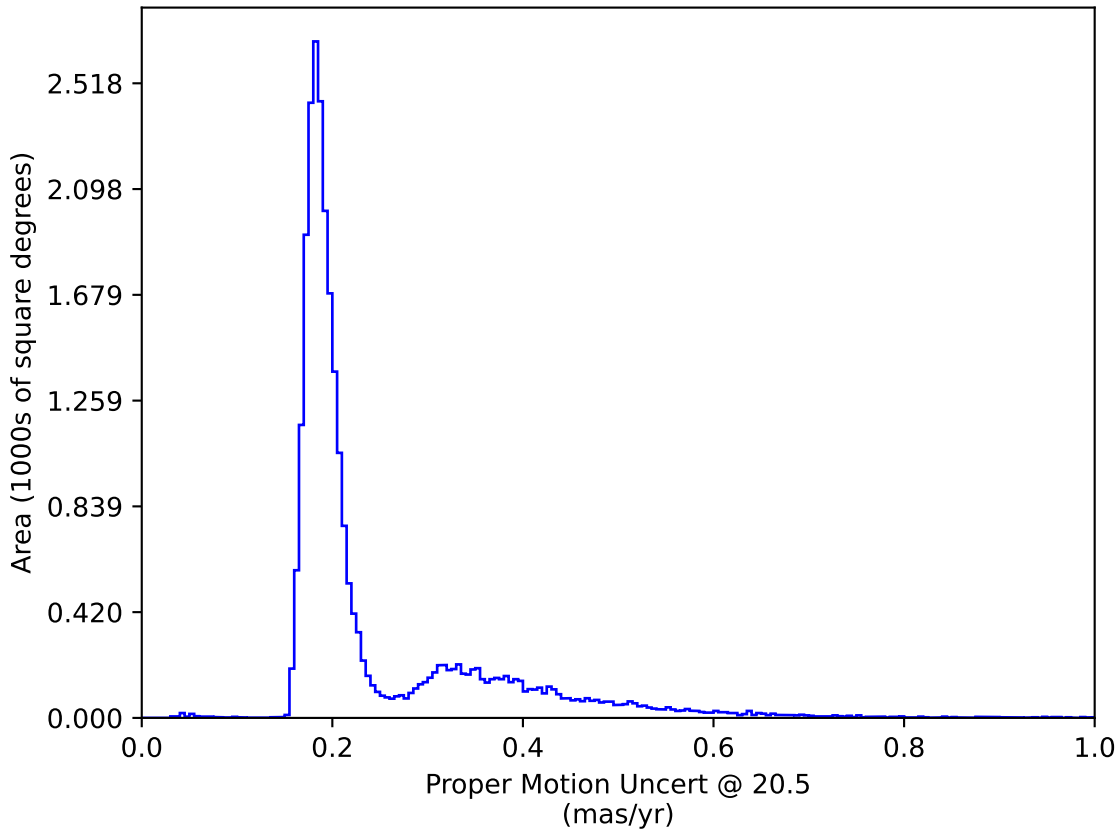
too_elab_r64_d2_giz_v3.4_10yrs : Proper Motion Uncert @ 20.5
