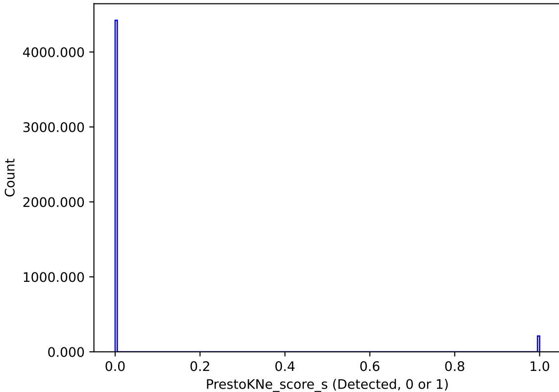
too_elab_r64_d2_giz_v3.4_10yrs : PrestoKNe_score_s
