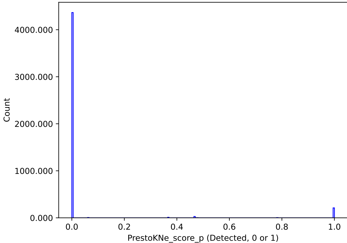
too_elab_r64_d2_giz_v3.4_10yrs : PrestoKNe_score_p
