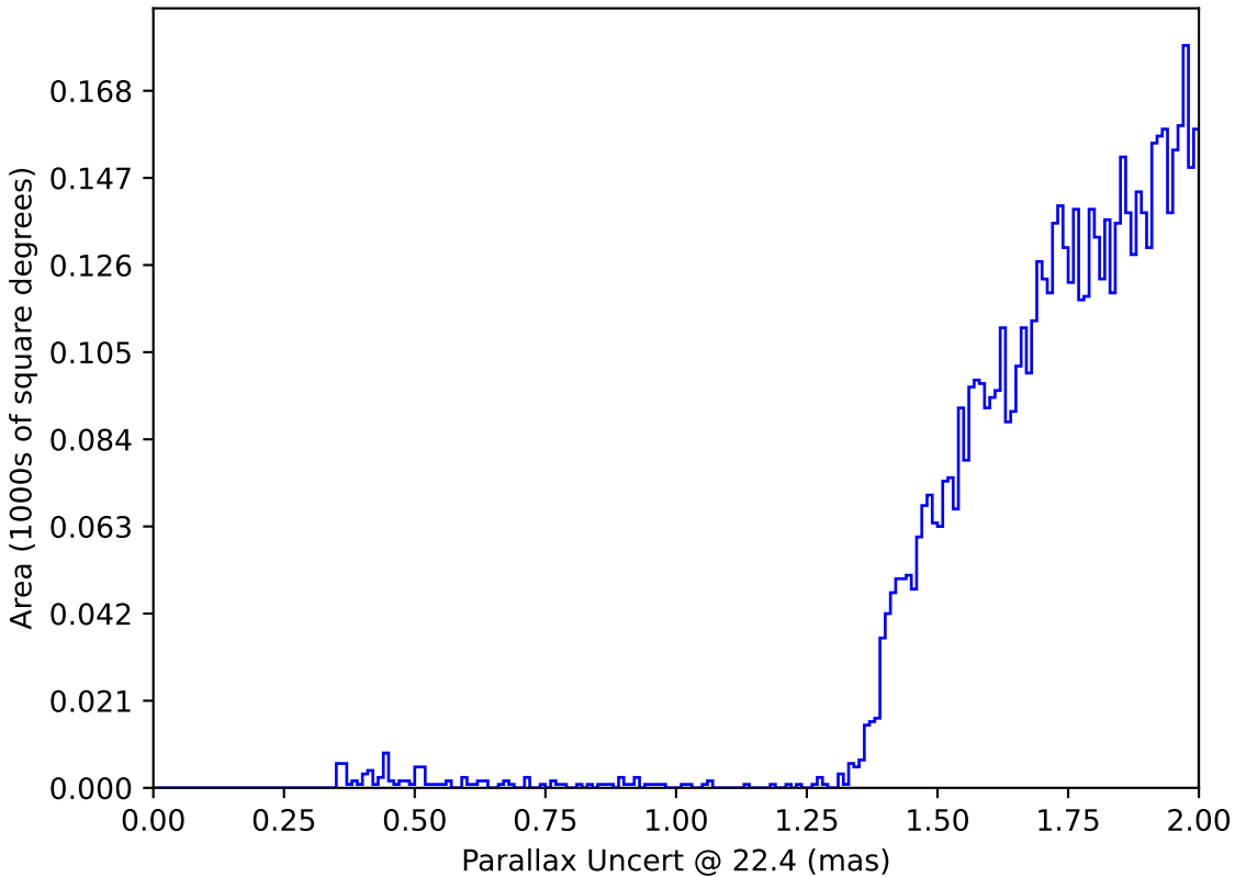
too_elab_r64_d2_giz_v3.4_10yrs : Parallax Uncert @ 22.4
