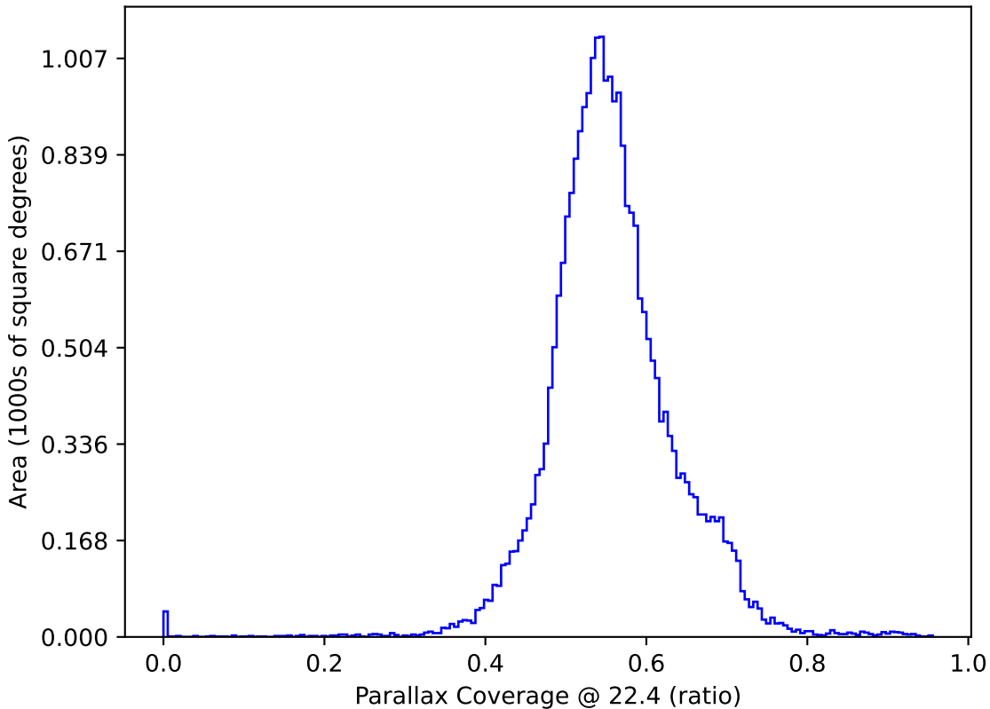
too_elab_r64_d2_giz_v3.4_10yrs : Parallax Coverage @ 22.4
