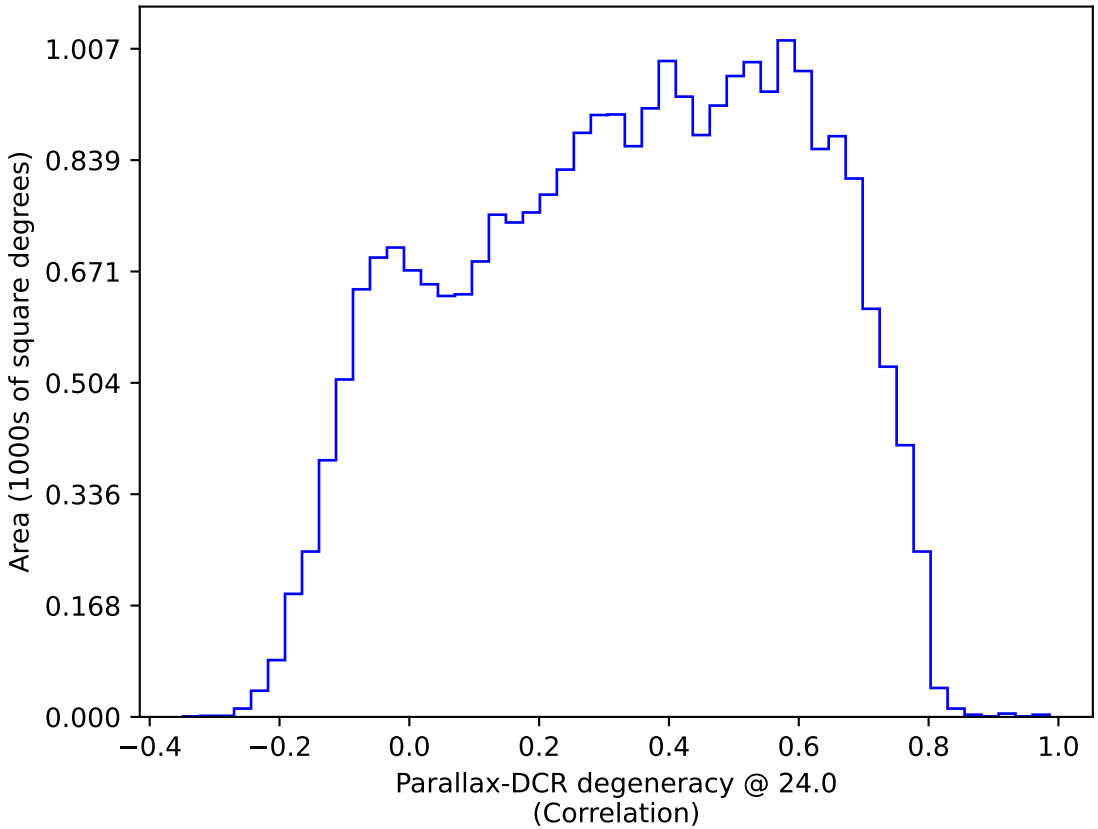
too_elab_r64_d2_giz_v3.4_10yrs : Parallax-DCR degeneracy @ 24.0
