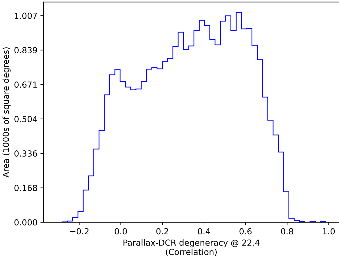
too_elab_r64_d2_giz_v3.4_10yrs : Parallax-DCR degeneracy @ 22.4
