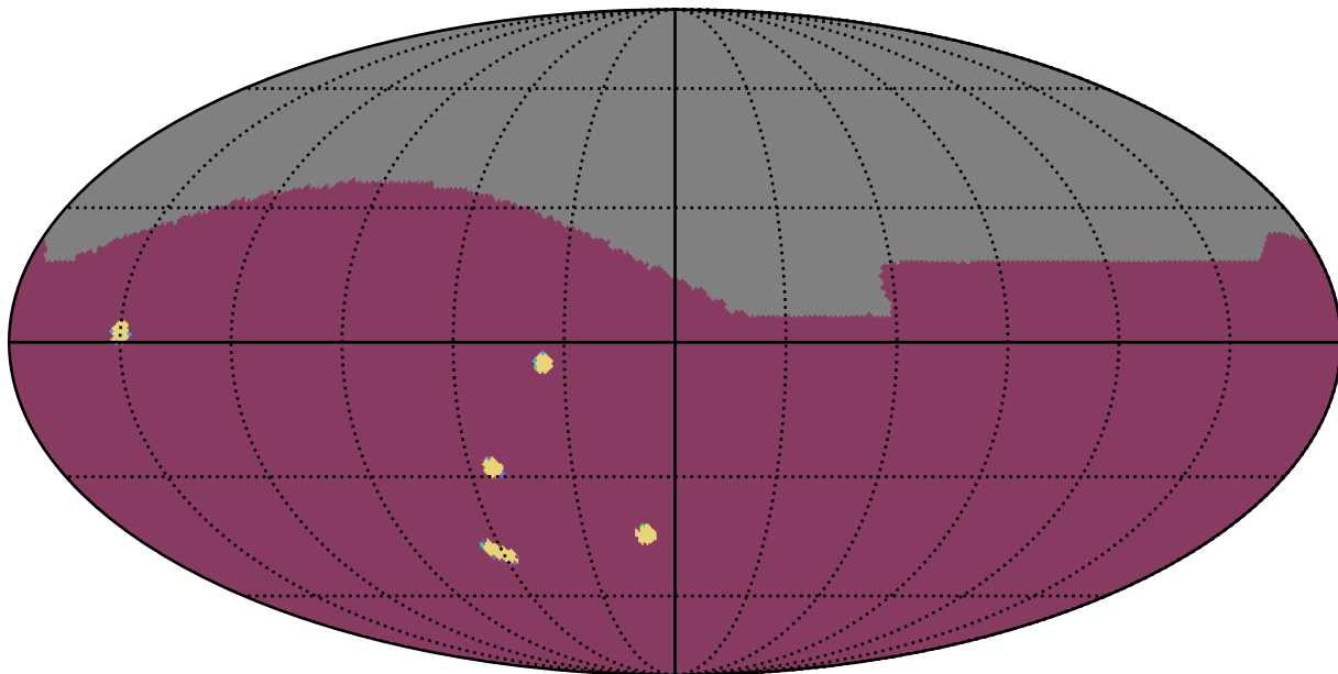
too_elab_r64_d2_giz_v3.4_10yrs : NumberOfQuickRevisits
