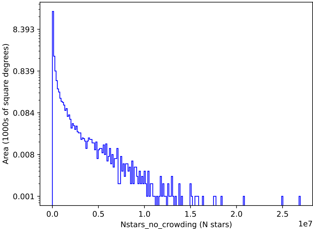
too_elab_r64_d2_giz_v3.4_10yrs z: Nstars_no_crowding
