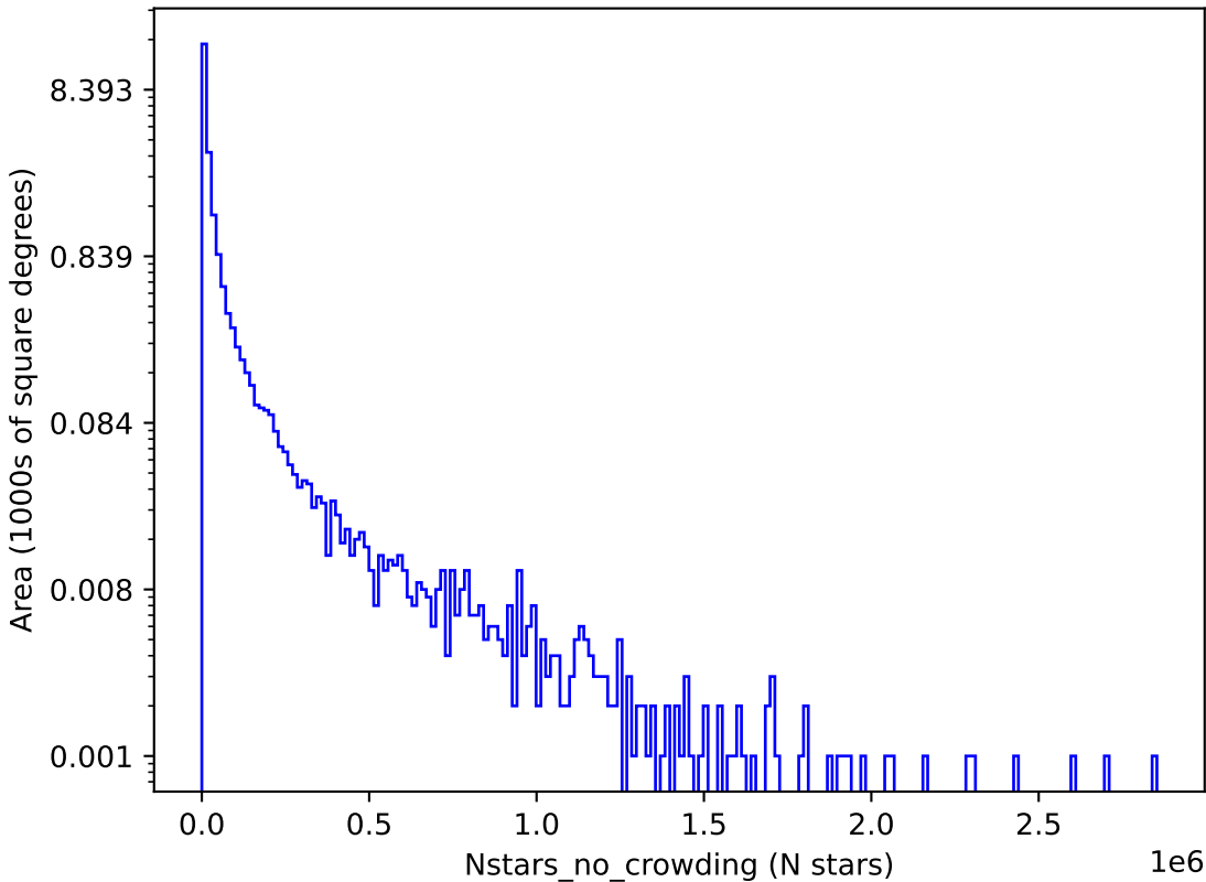
too_elab_r64_d2_giz_v3.4_10yrs u: Nstars_no_crowding
