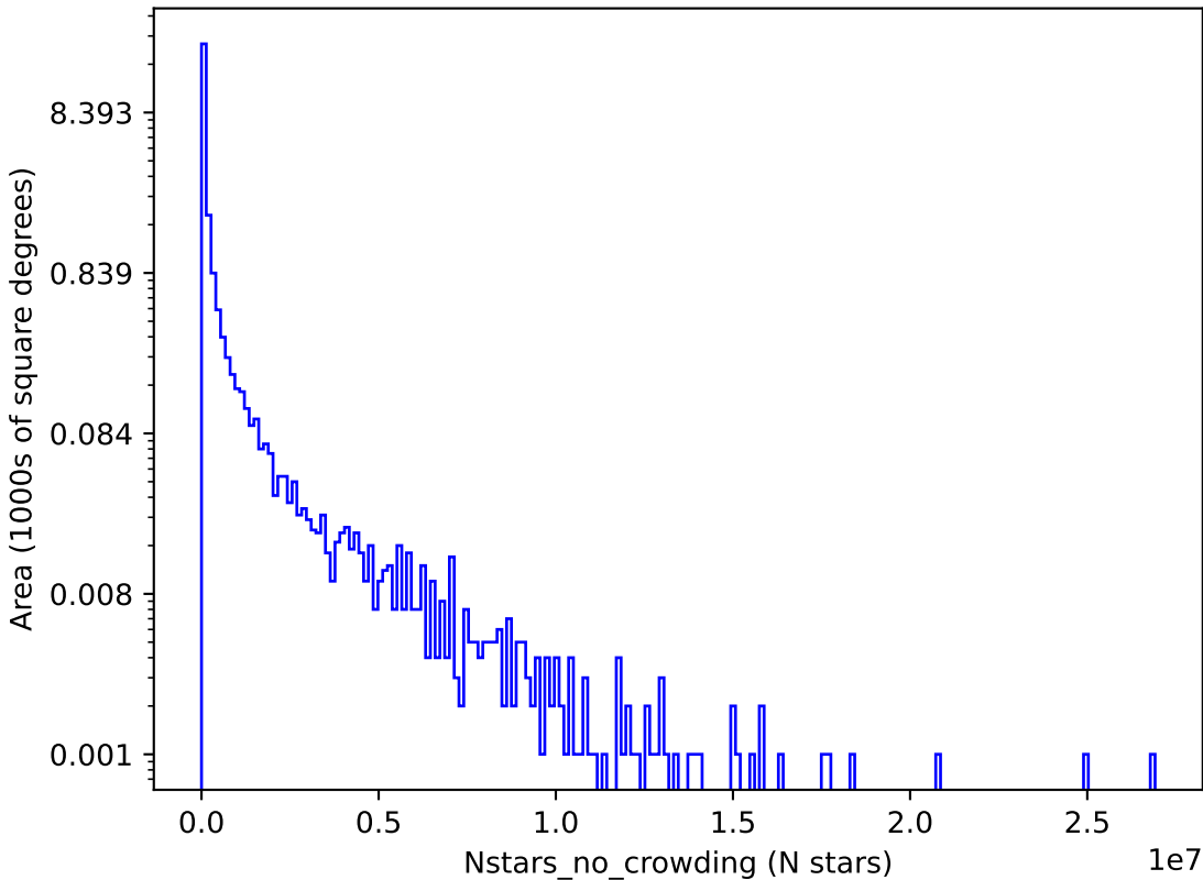
too_elab_r64_d2_giz_v3.4_10yrs i: Nstars_no_crowding
