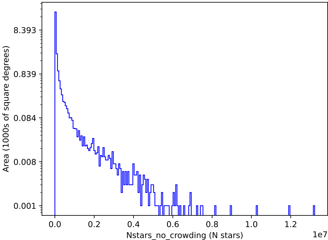
too_elab_r64_d2_giz_v3.4_10yrs g: Nstars_no_crowding
