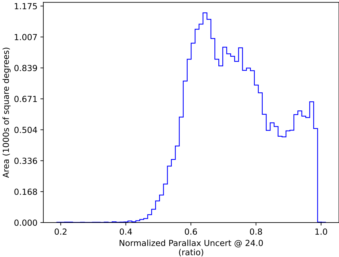
too_elab_r64_d2_giz_v3.4_10yrs : Normalized Parallax Uncert @ 24.0
