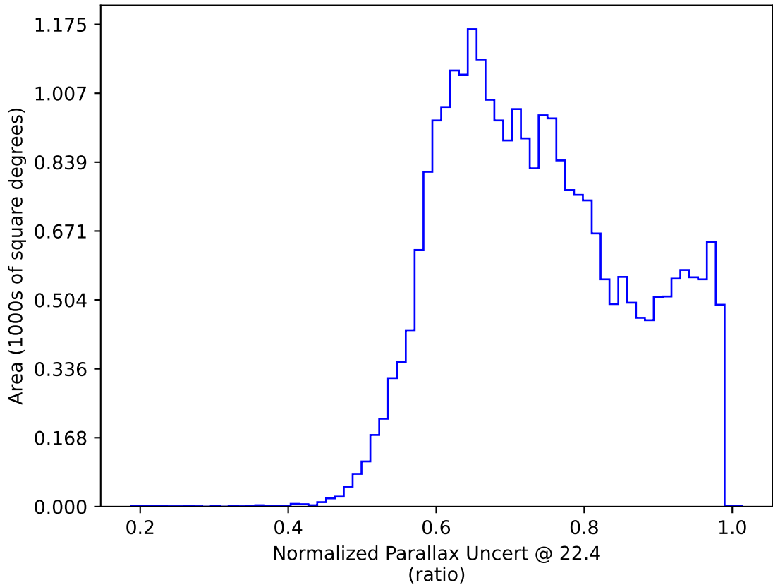
too_elab_r64_d2_giz_v3.4_10yrs : Normalized Parallax Uncert @ 22.4
