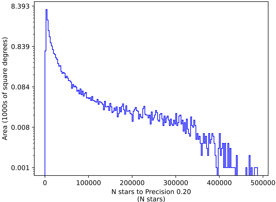
too_elab_r64_d2_giz_v3.4_10yrs u: N stars to Precision 0.20
