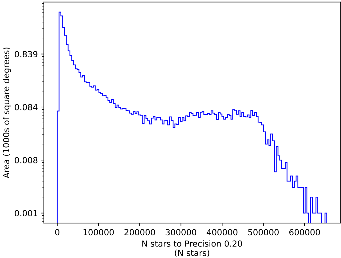
too_elab_r64_d2_giz_v3.4_10yrs r: N stars to Precision 0.20
