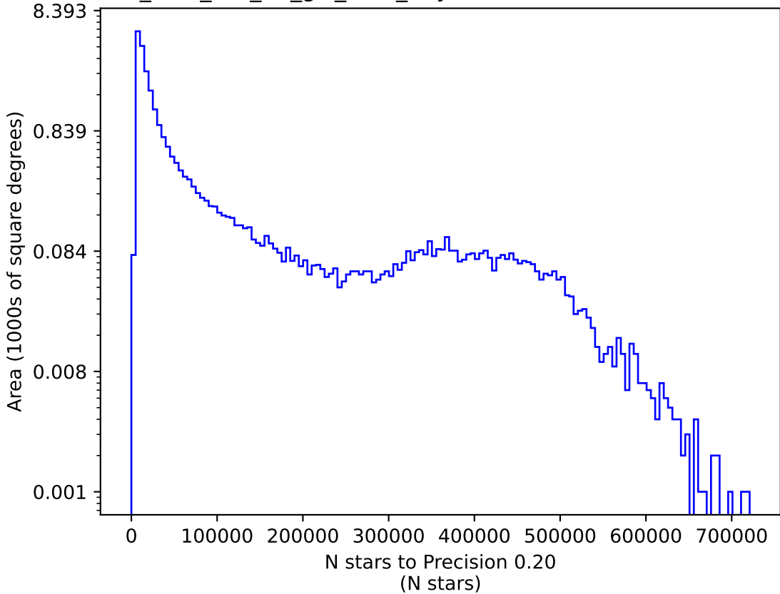
too_elab_r64_d2_giz_v3.4_10yrs i: N stars to Precision 0.20
