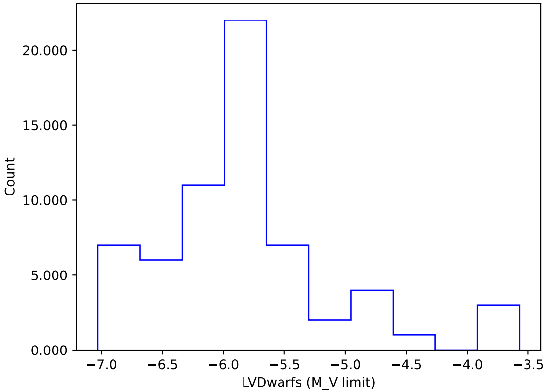
too_elab_r64_d2_giz_v3.4_10yrs gi: LVDwarfs
