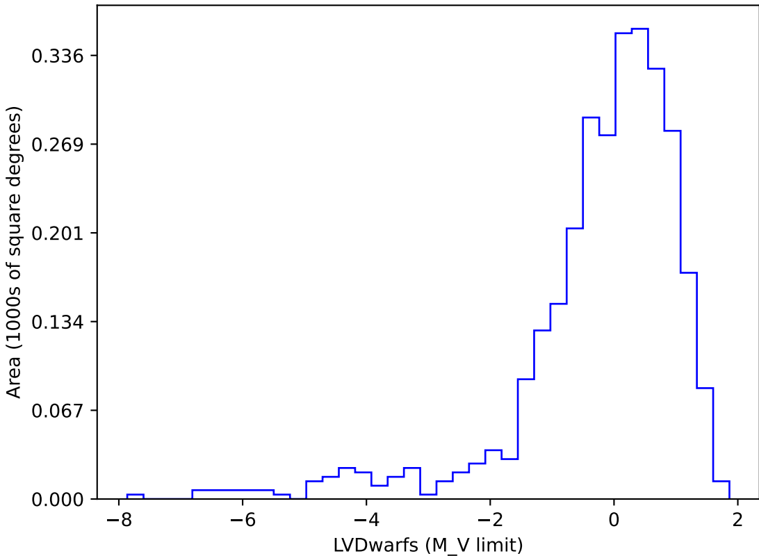
too_elab_r64_d2_giz_v3.4_10yrs gi SCP: LVDwarfs
