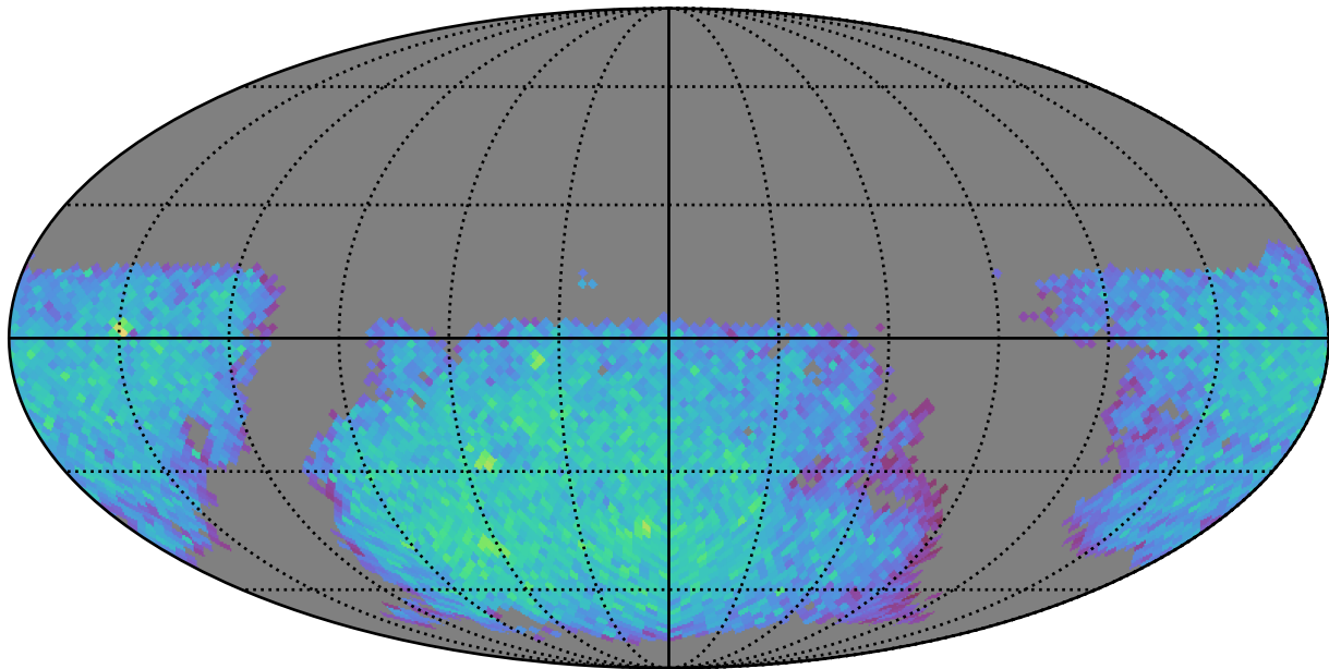
too_elab_r64_d2_giz_v3.4_10yrs gi: LVDwarfs
