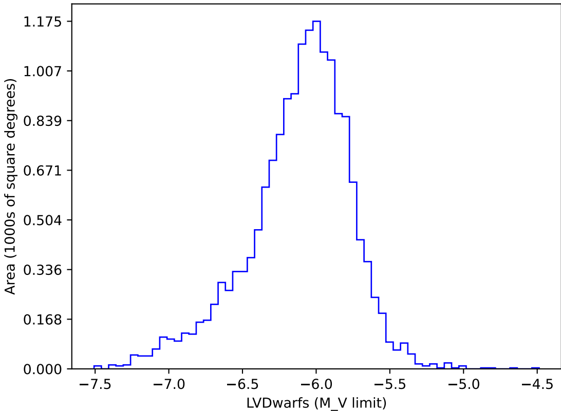
too_elab_r64_d2_giz_v3.4_10yrs gi: LVDwarfs
