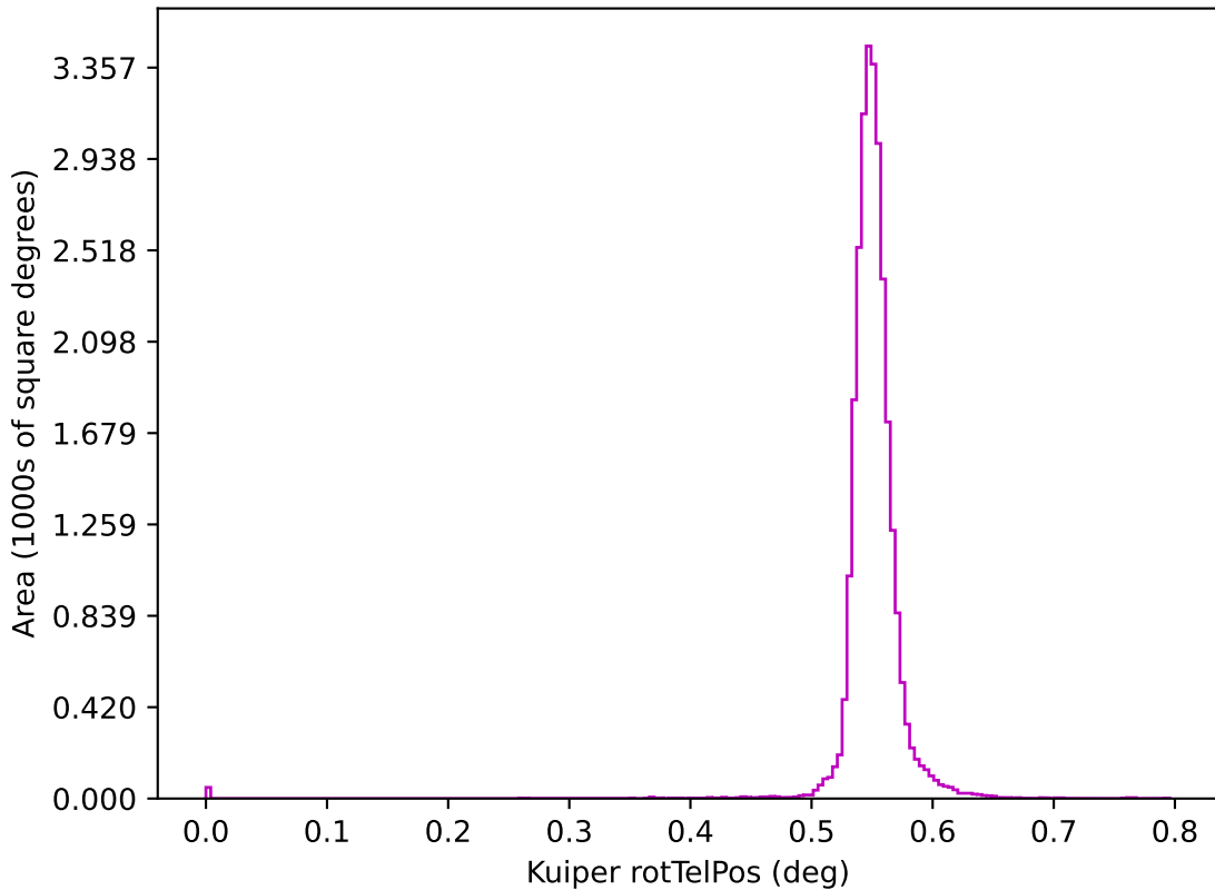
too_elab_r64_d2_giz_v3.4_10yrs z: Kuiper rotTelPos
